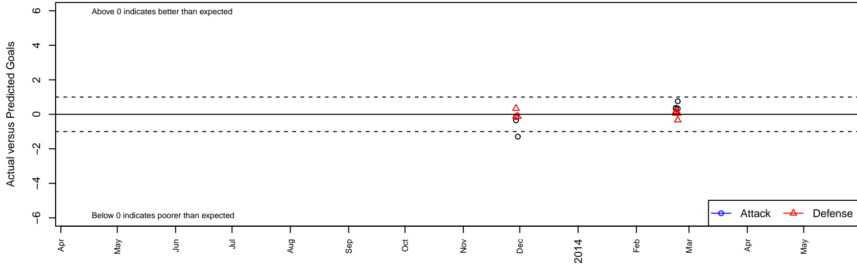
FC Bravo 01 B00 Dots are actual minus expected GF (blue circles) and GA (red triangles). Blue line is smoothed change in attack strength. Red is smoothed change in defense strength.
